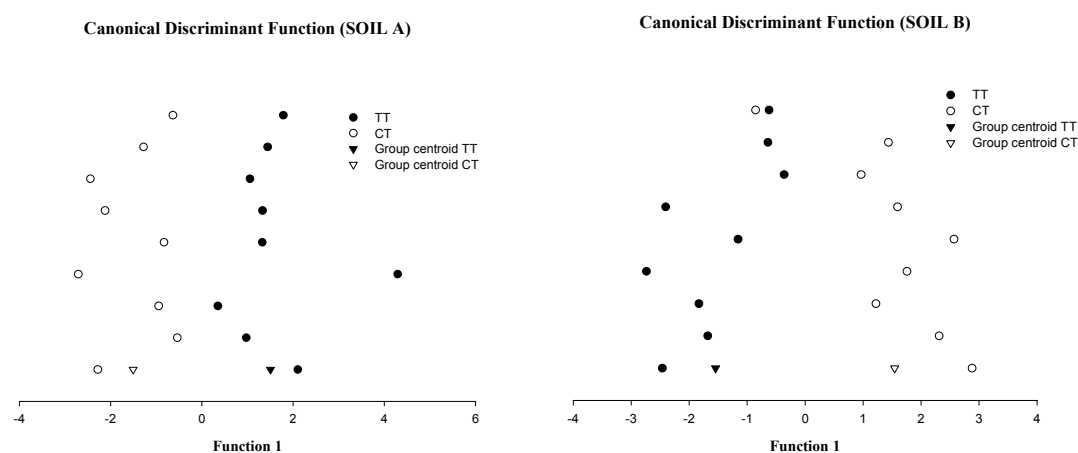
Figure 1. One-dimensional plot of the discriminant analysis of soil chemical and biochemical properties from soil under traditional tillage (TT) and conservation tillage (CT).
